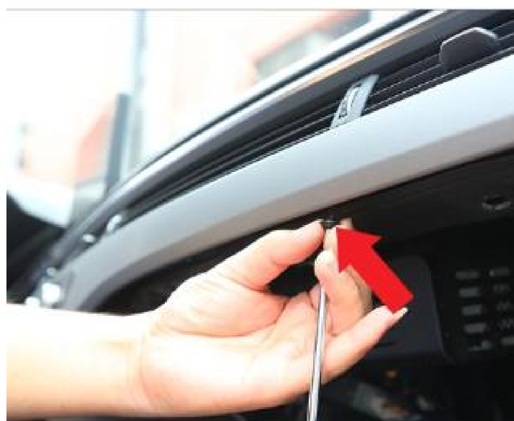
10. Remove the two screws located at the bottom of the glove box and then detach the glove box by pulling it downward.
