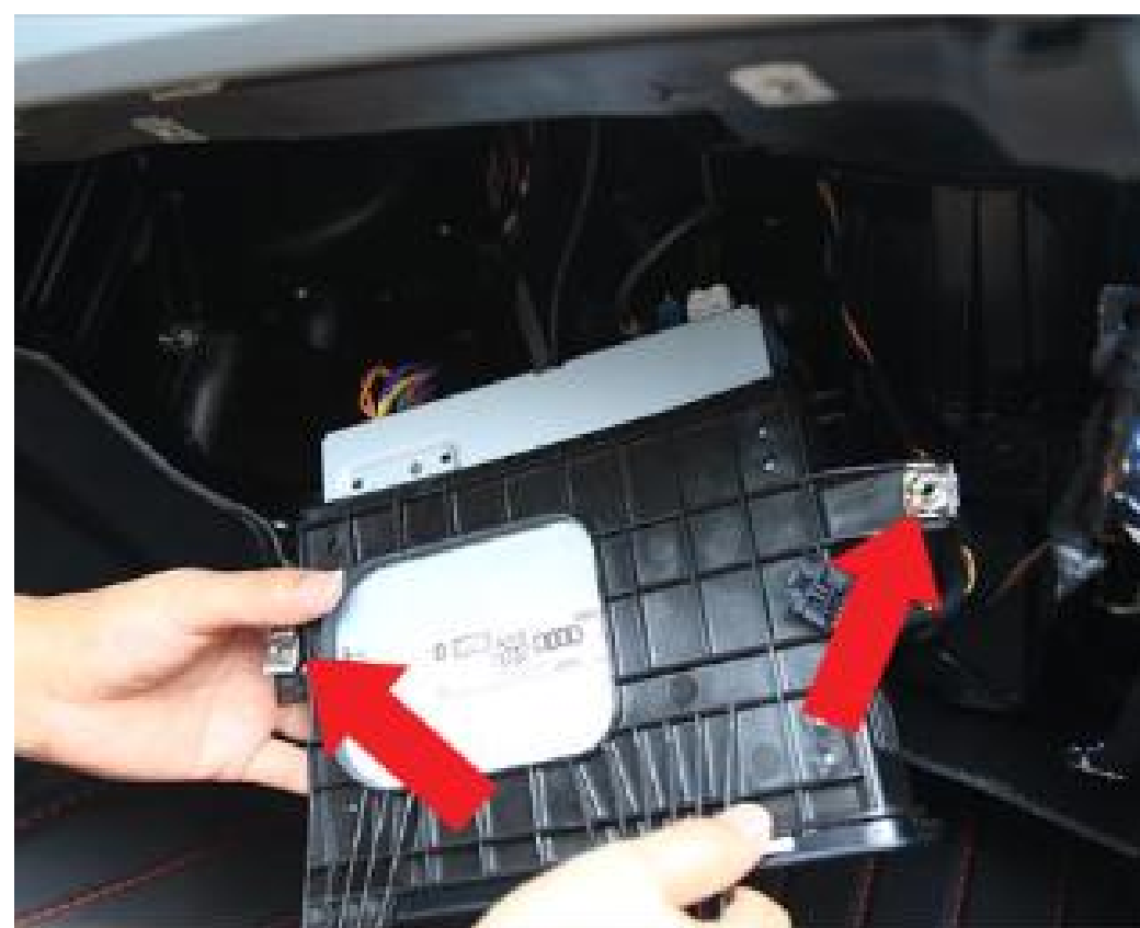
18. Remove the MIB head unit by unscrewing the holder screws.
