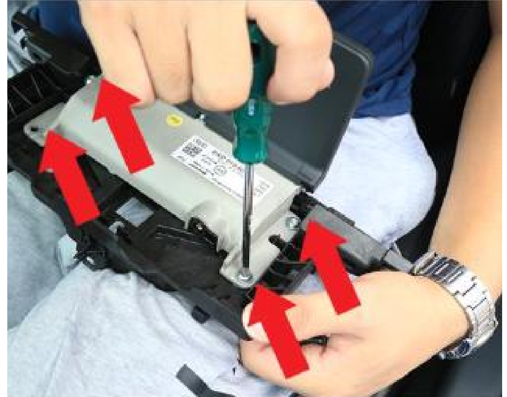
20. Unscrew the original screen from its tray.
